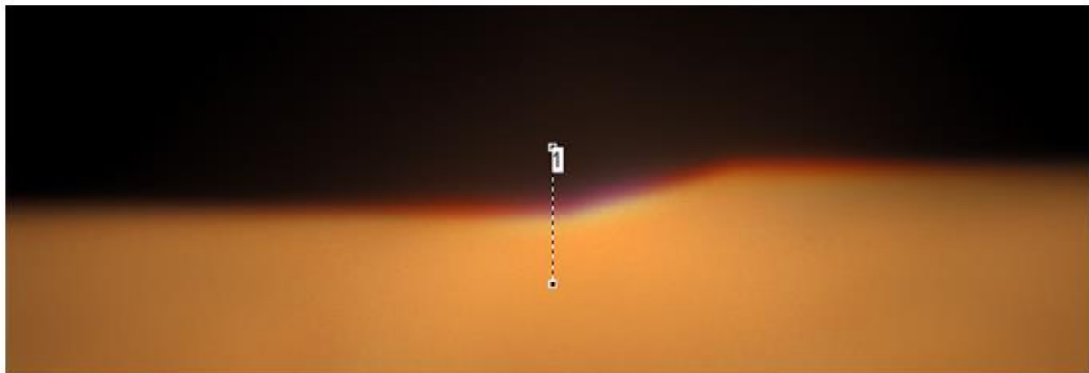
Figure 7: Color image of a halogen low beam with vertical section ( \pm 2^\circ ) at -0.5^\circ
