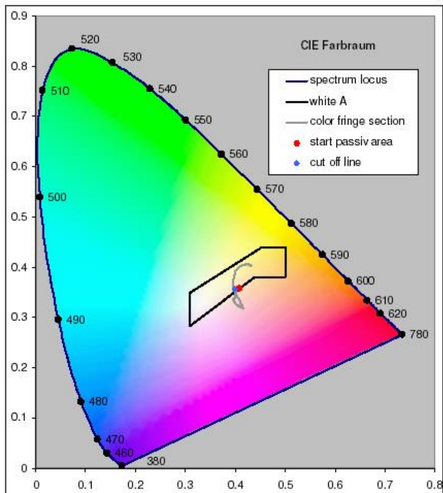
Figure 10: CIE color space with white region and section
